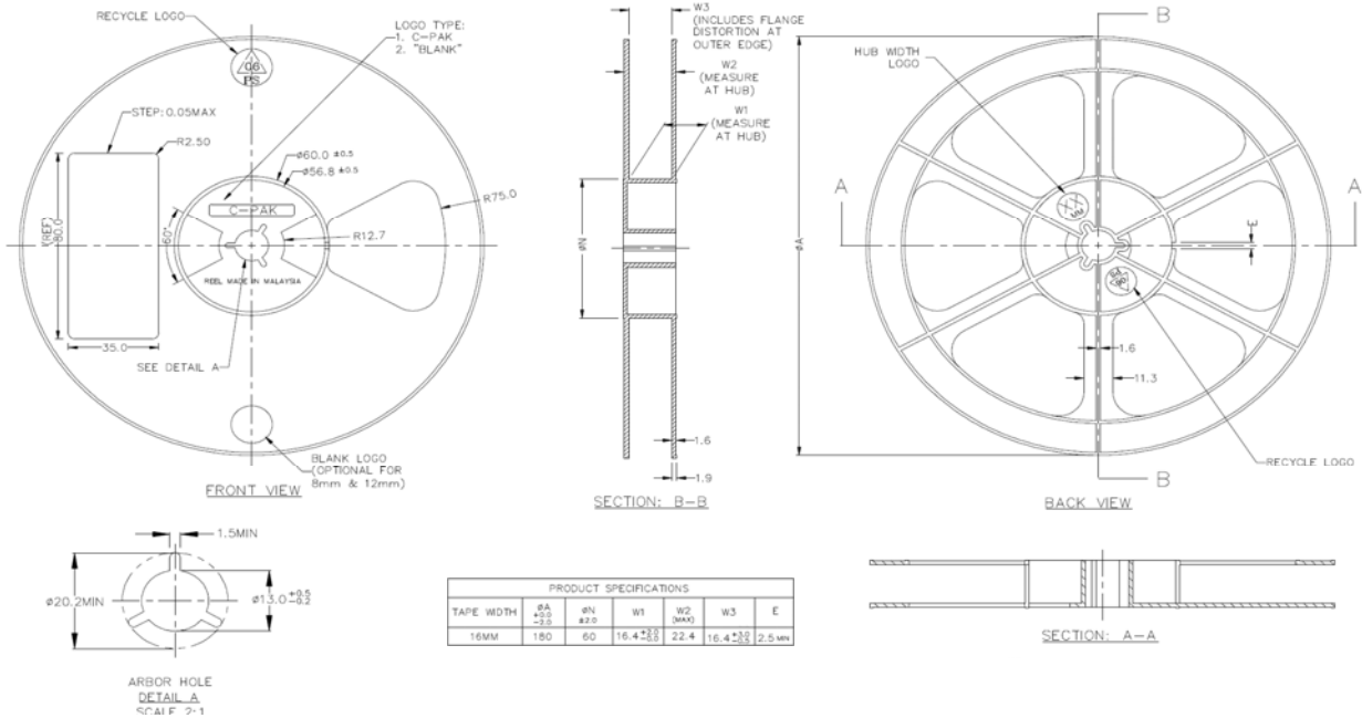
Figure 1: 7" Reel
