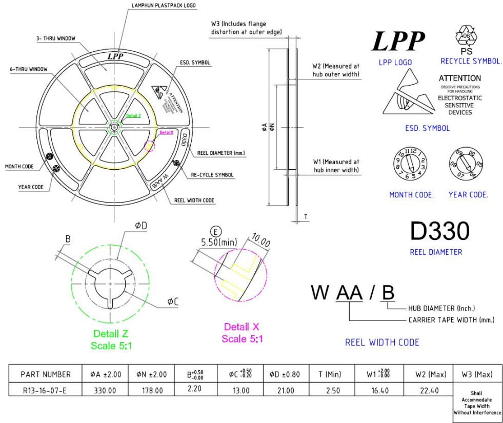
Figure 2: 13" Reel
