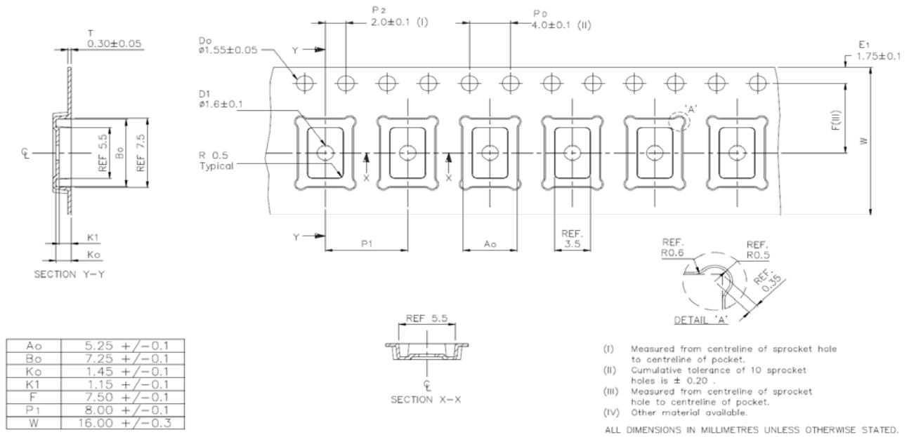
Figure 3. Embossed Carrier Tape
